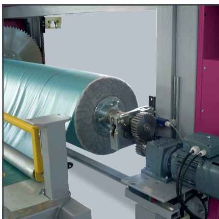
Motorized PVB/EVA unwinding device
