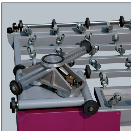
Single suction device (ER 100) as an additional equipment for small glass units
